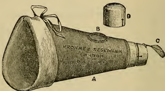
FIG. 26.—Krohne and Sesemann's Feather Register Cone.
